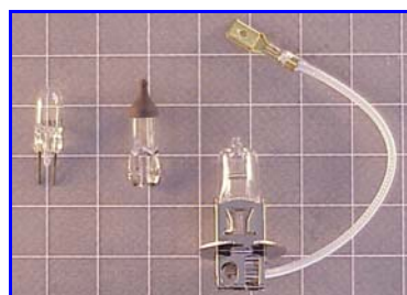
HB 891 1 HB 2040 1 HB 3 1 8 Watt 8 Watt 100 Watt
